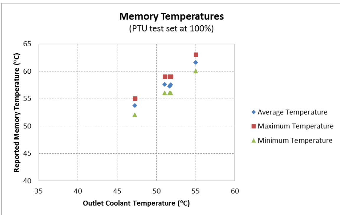
Figure 19. Memory temperature: PTU test set at 100%
